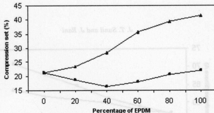
FIGURE 6 Variation of compression set with percentage of EPDM. ■, EPDM (B)/CIIR blends and ▲, EPDM (A)/CIIR blends.
