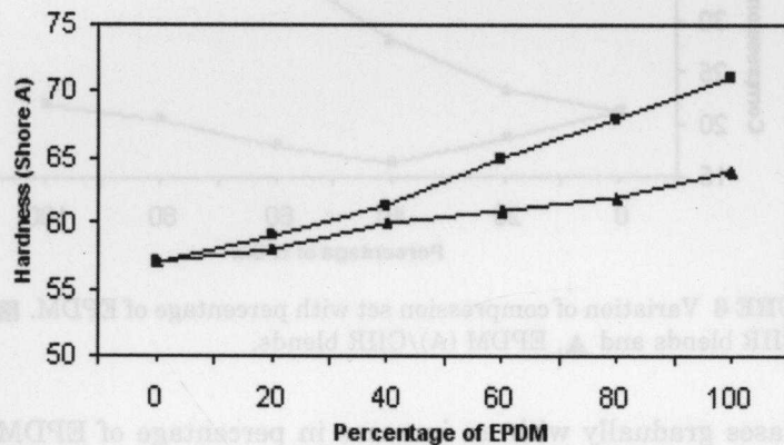
FIGURE 7 Variation of hardness with percentage of EPDM. ▲, EPDM (A)/CIIR blends and ■, EPDM (B)/CIIR blends.
