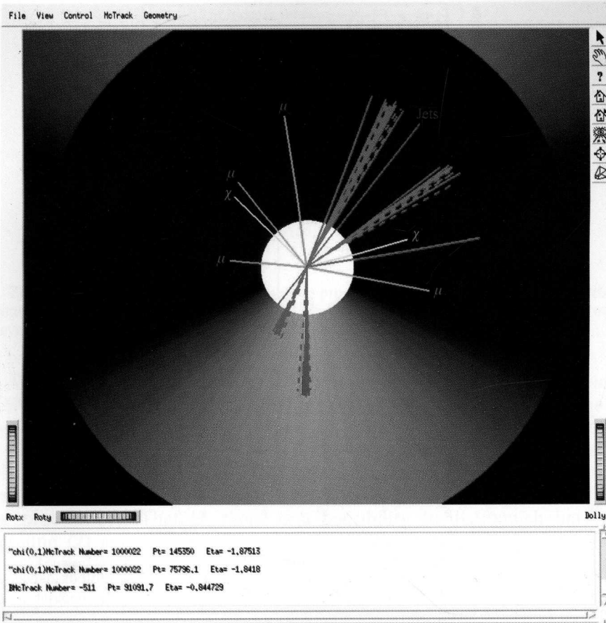
Fig. 3. Generation of the process 1 inside the cylindrical (Layer 1) pixel detector in the XY plane (transversely to the beam). One can see four muon tracks (green lines), two tracks from neutralino (light blue lines), four jets (dark blue lines) and one long-living B meson (red line). Visualisation has been performed with the help of ATLAS GeoModel HitDisplay [8]
