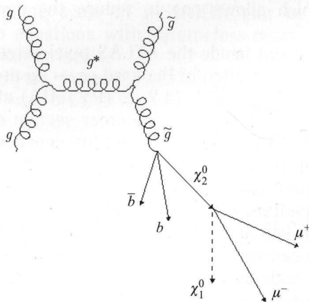
Fig. 2. Topology of the «half of the event» under study with two b jets, two muons and two secondary vertices
