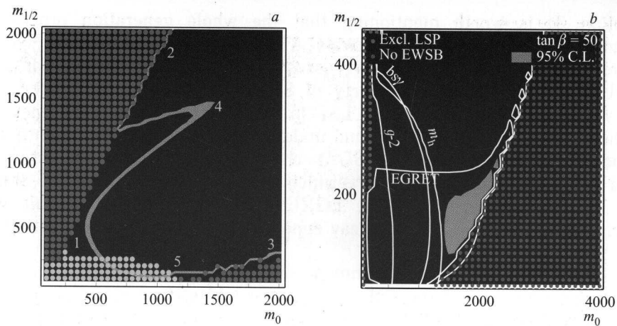
Fig. 1. a ) MSSM parameter space. Light blue line corresponds to the region consistent with WMAP data. One can distinguish between different regions marked by digits. 5 — is the EGRET region. b ) The light shaded (blue) area is the enlarged region preferred by EGRET data for \tan \beta = 50 , \mu > 0 and A_0 = 0 . The excluded regions where the stau would be the LSP, or the electroweak symmetry breaking fails, or the Higgs boson is too light, are indicated by dots
