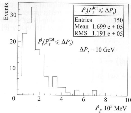
Fig. 5. Total missing transverse momentum P_t of two neutralinos. Event selection is made assuming that the total P_t of gluino pair is less than 10 GeV. Since in our study the initial state radiation was not taken into account, all events satisfy this condition
