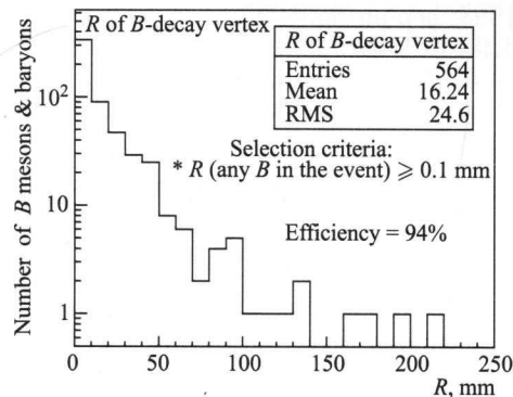
Fig. 6. The free path of B hadrons created in the process (1) before their decay. The criterion for the event selection is that the free path is not less than 100 \mu\text{m} for each of four B hadrons in the same event. 94% of events satisfy this condition
