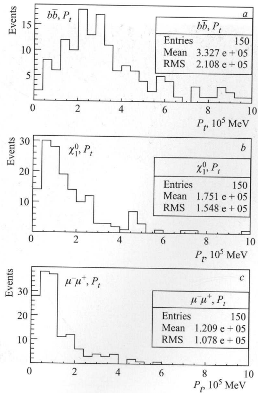
Fig. 4. Transverse momentum distributions for the products of one of the gluinos decay. a) The total P_t for the b\bar{b} pair; b) P_t for the lightest stable neutralino \tilde{\chi}_1^0 from the heavier neutralino decay; c) total P_t for the muon pair
