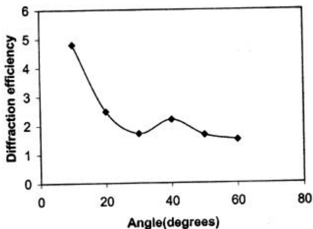
Figure 10. A plot of diffraction efficiency vs angle.
