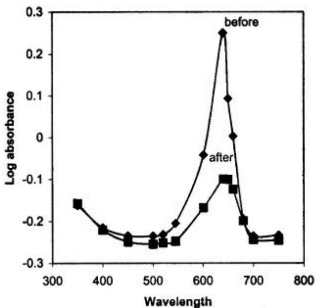
Figure 1. Optical absorption spectra of CMBPVC film for a pH of 4.5 before and after exposure.
