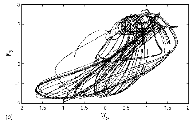
FIG. 2. (a) The outer junctions are synchronized. (b) The outer junction and middle junction are uncorrelated. The parameter values are \beta=0.3 , i_0=1.2 , \Omega=0.6 , i_{dc}=0.3 , \alpha_s=0.37 .
