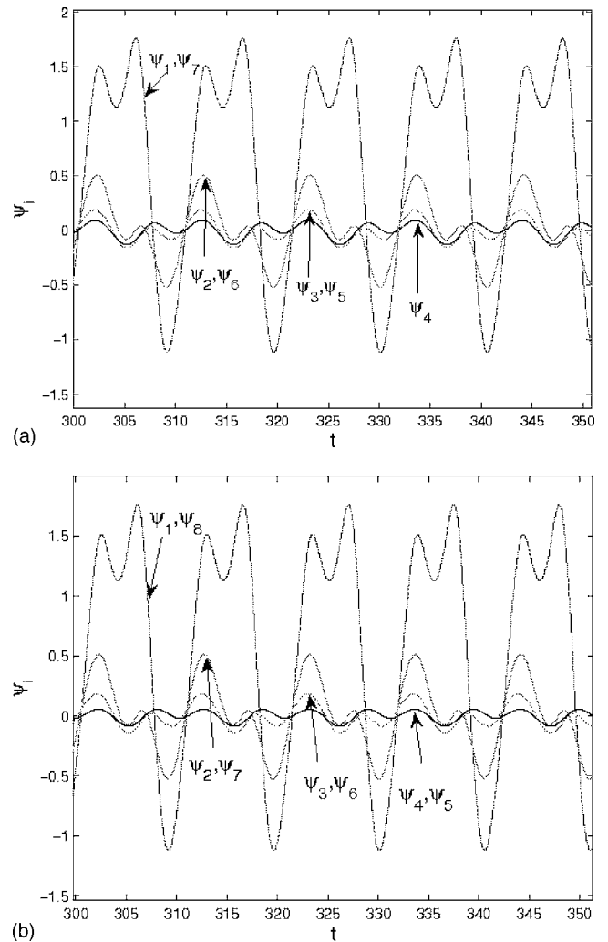
FIG. 4. (a) The time series plot for an array of seven JJs and (b) for eight junctions. \beta=0.3 , i_0=1.2 , \Omega=0.6 , i_{dc}=0.3 , \alpha_s=0.37 and \theta=0.5\pi .
