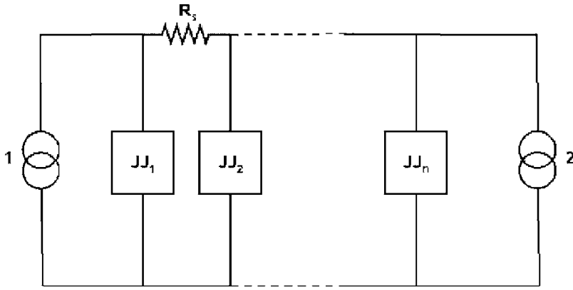
FIG. 1. Schematic representation of an array of JJ linked in parallel with a linking resistor R_s . 1 and 2 are the driving fields.
