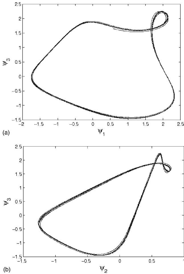
FIG. 3. (a) and (b) show that the junctions are phase correlated. \beta=0.3 , i_0=1.2 , \Omega=0.6 , i_{dc}=0.3 , \alpha_s=0.37 , and \theta=0.5\pi .
