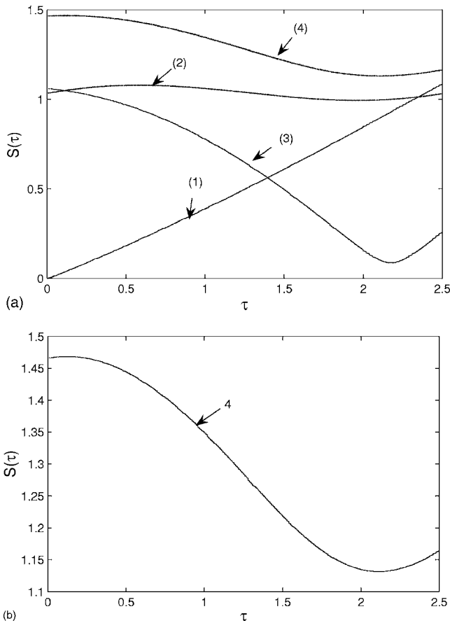
FIG. 5. (1) is S(\tau) for variables \psi_1 and \psi_3 , (2) for \psi_1 and \psi_2 . Line (1) shows complete synchronization while the other is not synchronized. Both these lines are plotted with no phase difference applied. (3) and (4) give the similarity function for the variables. \psi_1 and \psi_3 , and \psi_1 and \psi_2 in the presence of phase difference \theta=0.5\pi . The second figure shows line 4 where the dip can be observed clearly.
