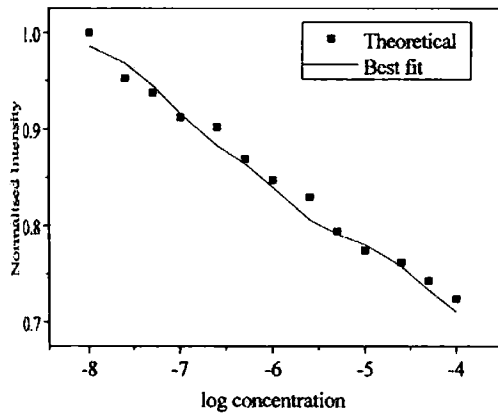
Fig. 4. Plot showing cladding-mode intensity variation with dye.
