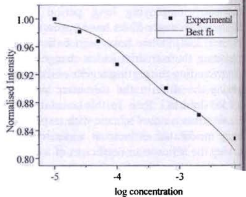
Fig. 3. Plot showing core-mode intensity variation with concentration.
