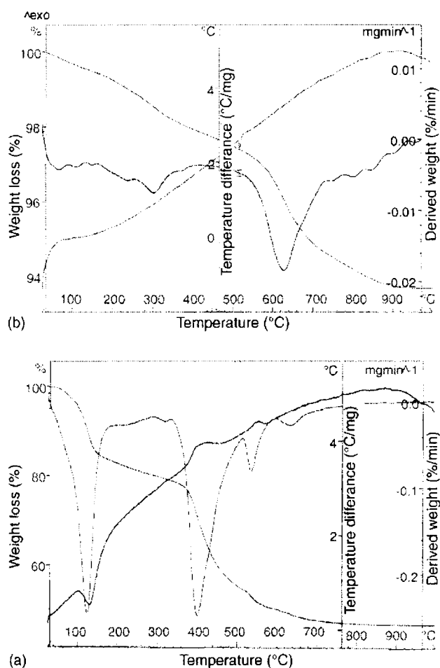
Fig. 5. Thermo gravimetric-differential thermal analysis (TG-DTG, DTA) plots of: (a) 3VN/100 and (b) 15VN/500.
