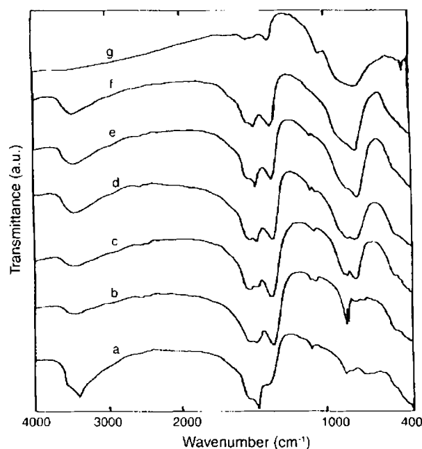
Fig. 3. FTIR spectra of: (a) 0VN/500, (b) 3VN/500, (c) 6VN/500, (d) 9VN/500, (e) 15VN/500, (f) NdVO_4 and (g) V_2O_5 .
