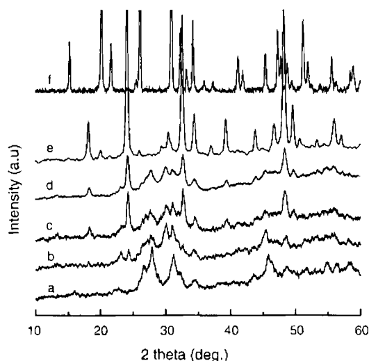
Fig. 1. Powder XRD patterns of V_2O_5 - Nd_2O_3 catalysts calcined at 500^\circ C : (a) 0VN/500, (b) 6VN/500, (c) 9VN/500, (d) 15VN/500, (e) NdVO_4 and (f) V_2O_5 .
