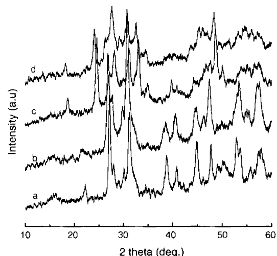
Fig. 2. Powder XRD patterns of V_2O_5 - Nd_2O_3 catalysts calcined at 700^\circ C : (a) 0VN/500, (b) 6VN/500, (c) 9VN/500 and (d) 15VN/500.
