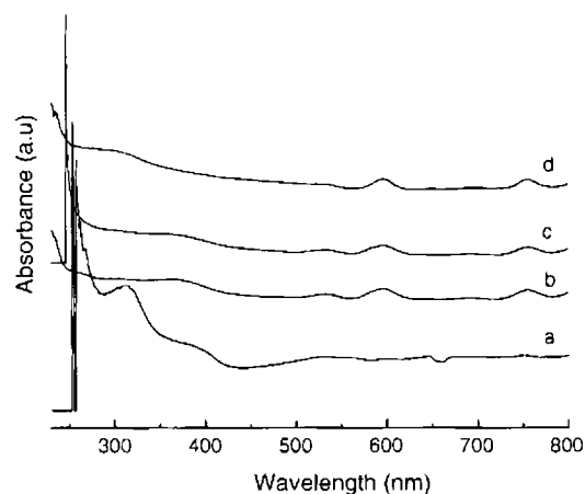
Fig. 4. Diffuse reflectance UV-Visible spectra of: (a) 0VN/500, (b) 6VN/500, (c) 12VN/500 and (d) \text{NdVO}_4 .
