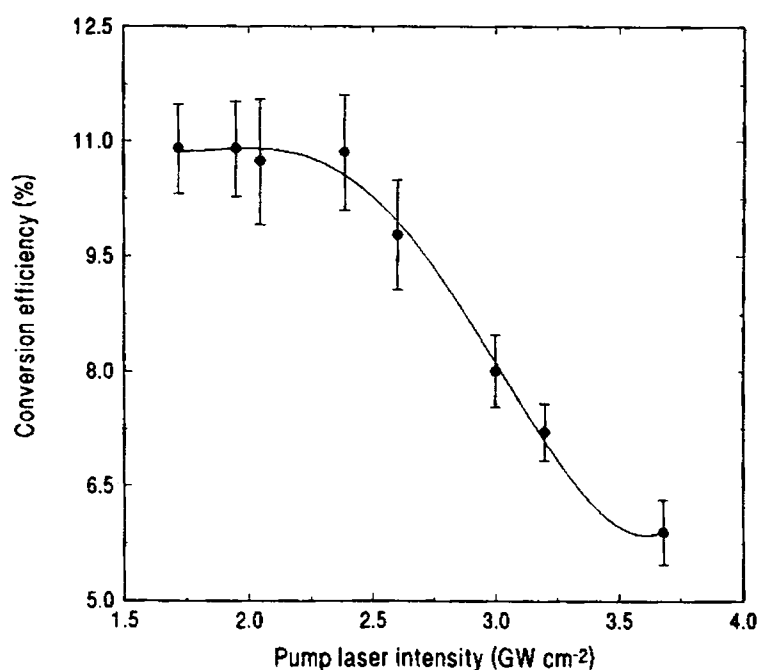
Fig.3.8 Plot of conversion efficiency as a function of laser intensity. Maximum single pass conversion efficiency is 11%
