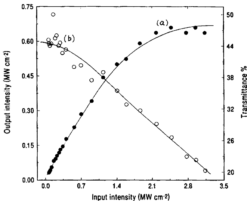
Fig.7.1 Plot of optical limiting observed in \text{Eu}(\text{Pc})_2 along with the transmittance curve
