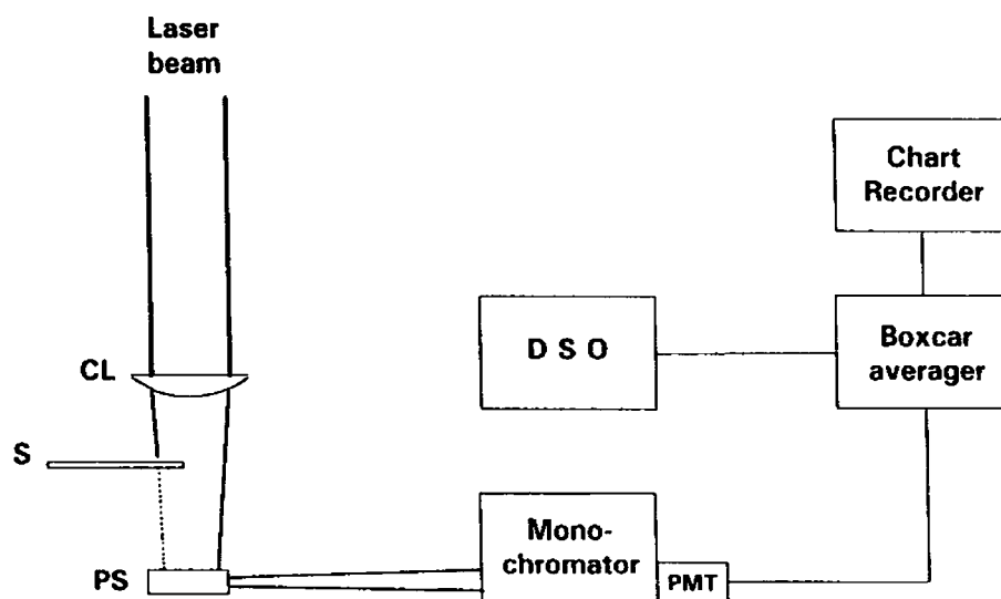
CL-Cylindrical lens, S-Shutter, PS-Polyacrylamide sample, PMT-Photomultiplier tube. DSO-Digital storage oscilloscope.
