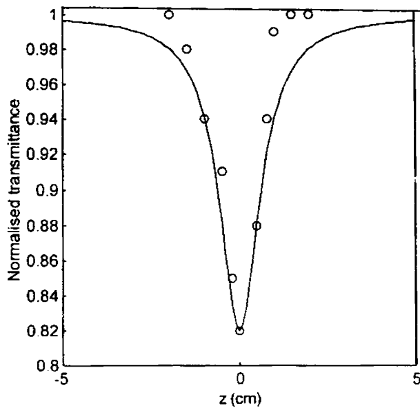
Fig.5.10 Open aperture trace of \text{Eu}(\text{Nc})_2 at 514.5 nm. From the theoretical fit, the value of \beta was found to be 787 cm/W.
