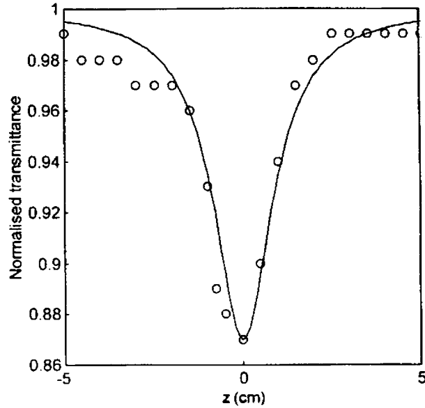
Fig.5.5 Open aperture Z-scan curve for \text{Eu}(\text{Pc})_2 at 514.5 nm. The solid line shows the theoretical fit, from which the value of \beta was found to be 187.03 cm/W.
