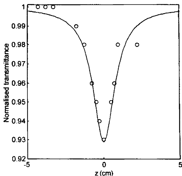
Fig.5.4 Open aperture Z-scan curve of \text{Eu}(\text{Pc})_2 at 476.5 nm. The solid line shows the theoretical fit with the value of \beta equal to 125.1 cm/W.
