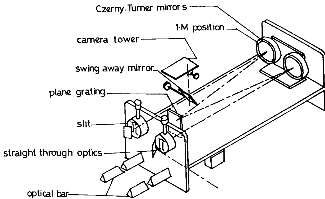
Fig.2.4 Optical layout of the Spex monochromator
