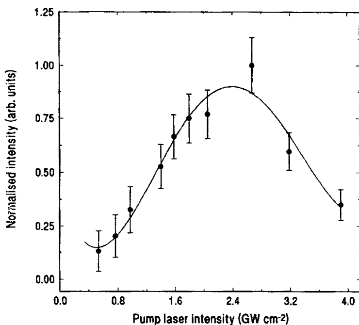
Fig.3.5 Wavelength integrated ASE intensity as a function of pump laser intensity. The decrease in emission intensity beyond 2.7 \text{ GW cm}^{-2} is due to nonlinear phenomena like excited state absorption, and two photon absorption
