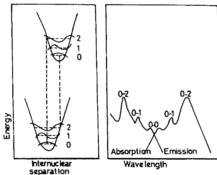
Fig.1.3 Mirror image rule and Franck-Condon factors.
