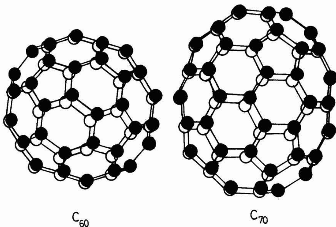
Fig.1.9 Chemical structure of the fullerenes C 60 and C 70
