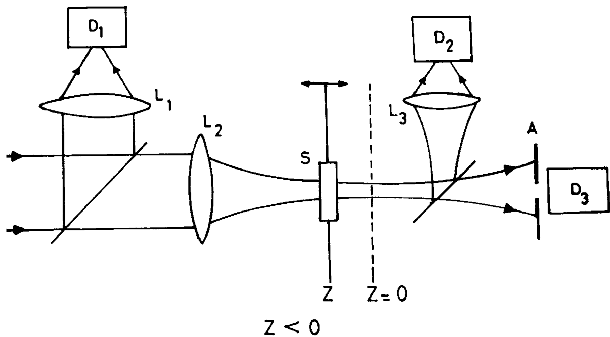
D_1, D_2, D_3 -Detectors, L_1, L_2, L_3 -Lens, S -Sample, A -Aperture Fig.1.6 Experimental setup for Z-scan technique.
