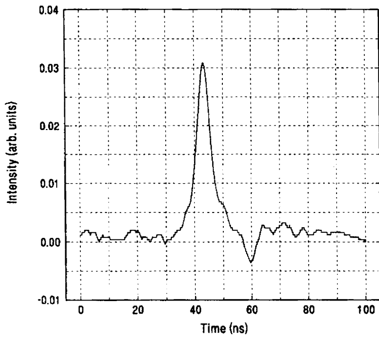
Fig.3.9 The temporal profile of the ASE pulse at a laser intensity of 0.2 \text{ GWcm}^{-2} . The pulsewidth is approximately 6 ns
