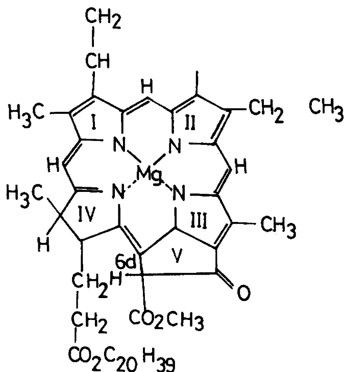
Fig.1.8 Chemical structure of Chlorophyll
