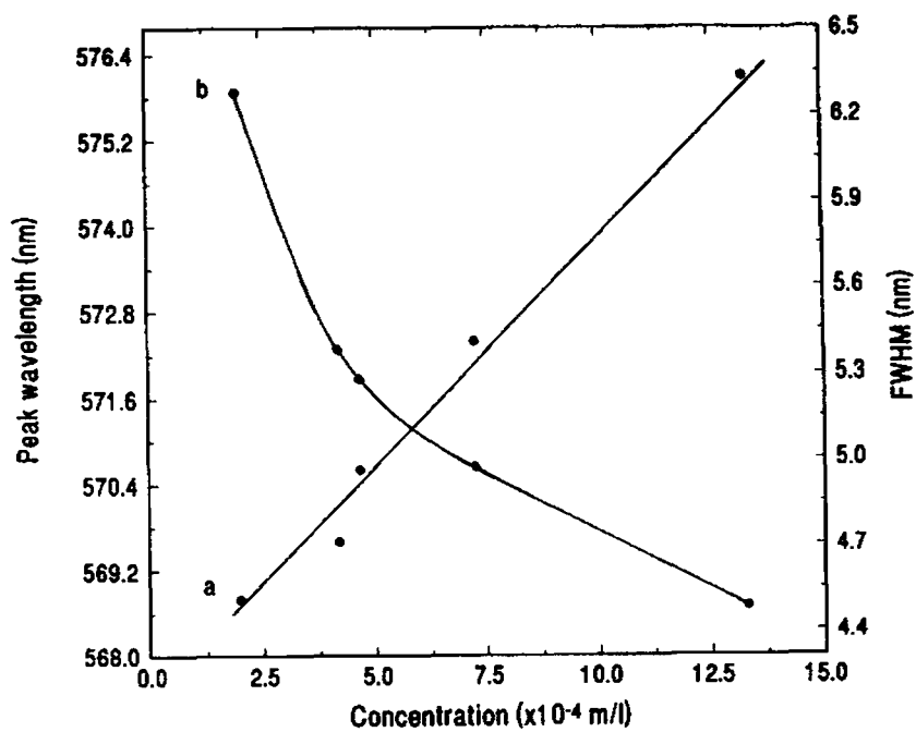
Fig.3.12 Variation of ASE peak wavelength (a) and spectral width (b) as a function of the concentration of dye
