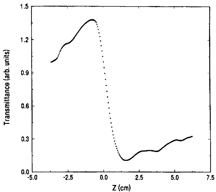
Fig.5.7 Closed aperture Z-scan trace at a pump wavelength of 514.5 nm. The nonlinear refractive index was measured as 4.5 \times 10^{-4} .
