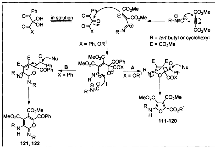
Scheme 37
