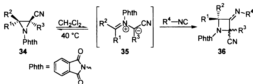
Scheme 15
