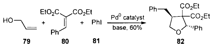
Scheme 24
