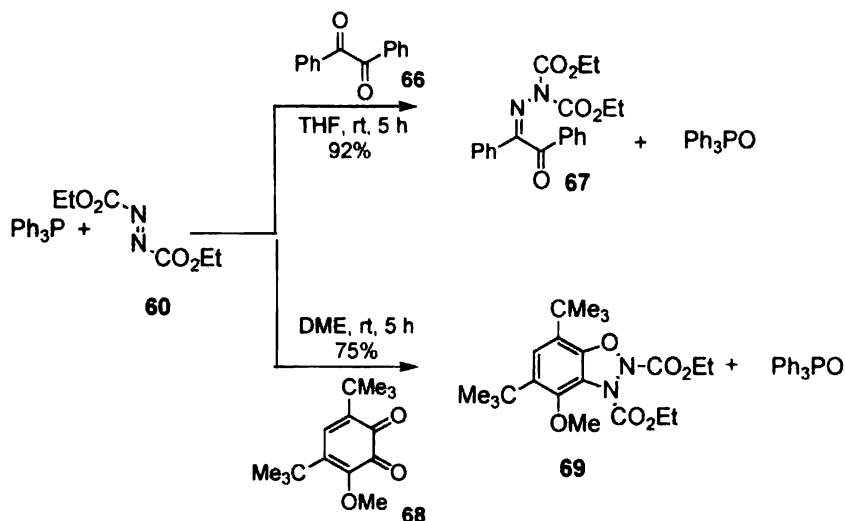
Scheme 24
