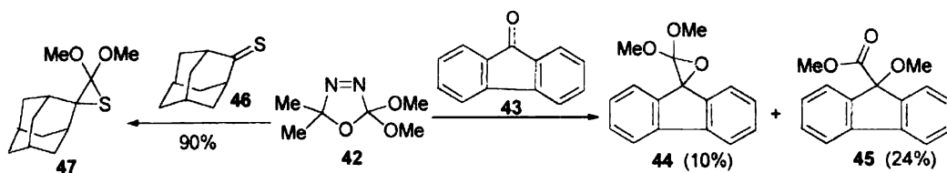
Scheme 10
