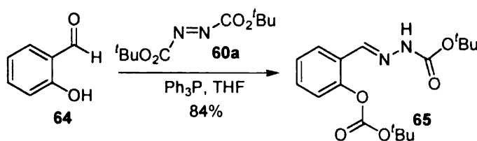
Scheme 23
