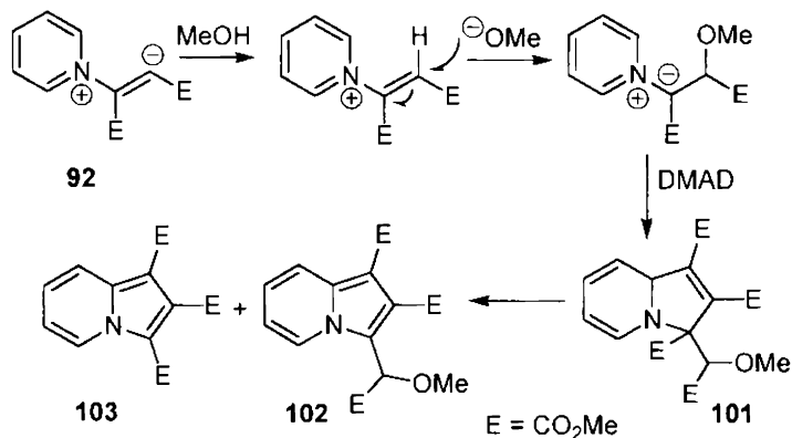
Scheme 30
