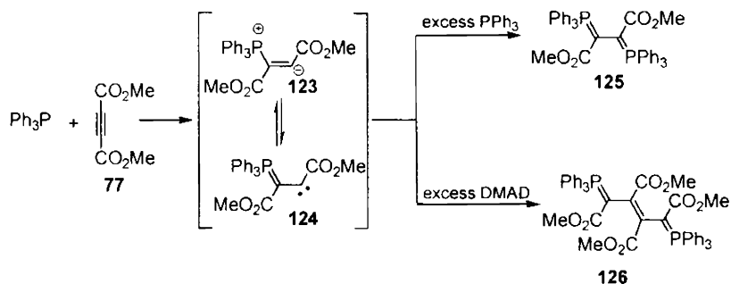
Scheme 40
