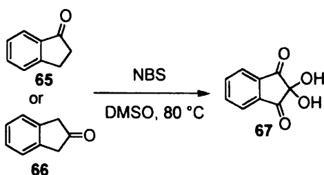
Scheme 23
