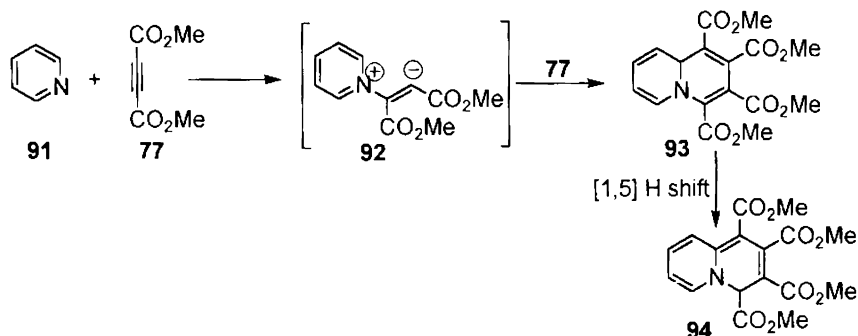
Scheme 27
