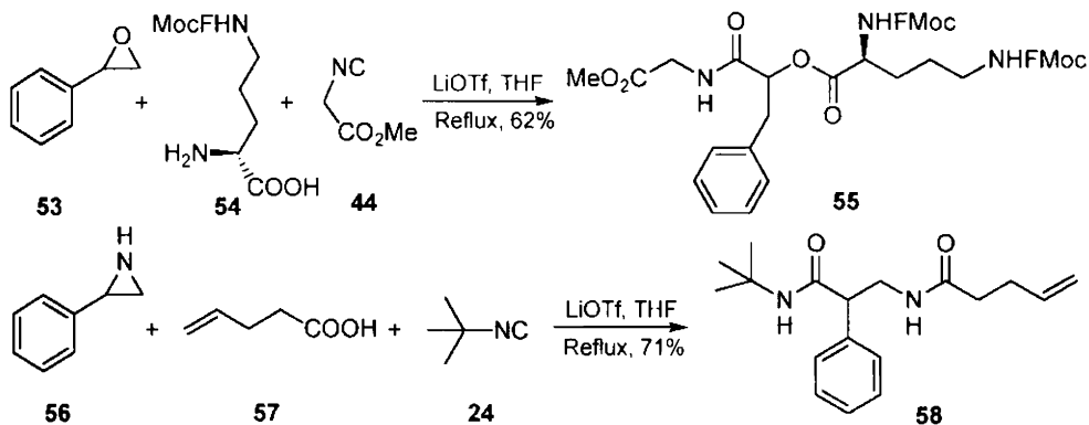
Scheme 17
