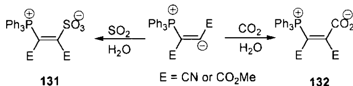
Scheme 43
