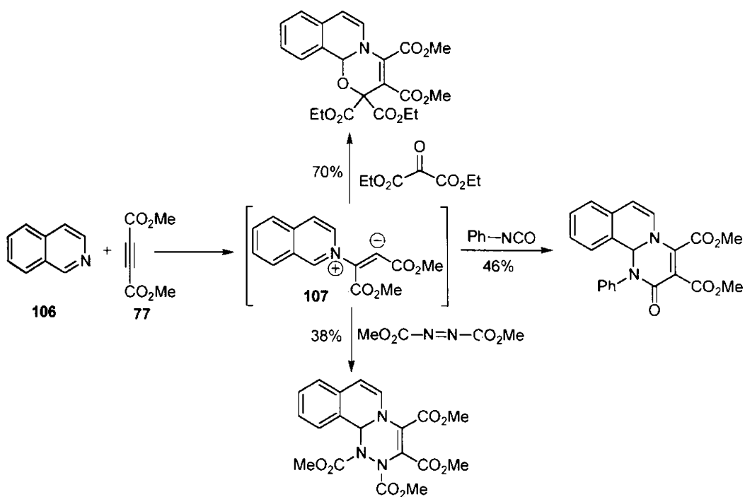
Scheme 33
