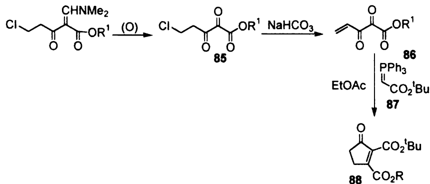
Scheme 28
