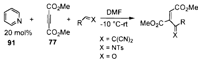
Scheme 31
