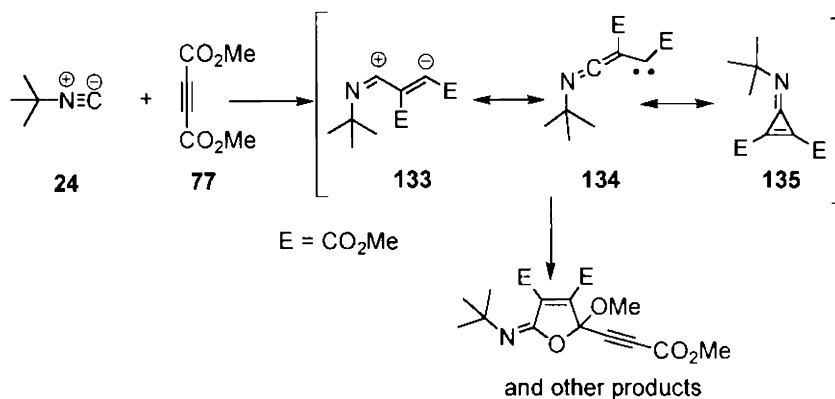
Scheme 44
