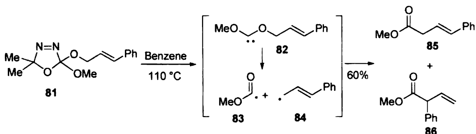
Scheme 21
