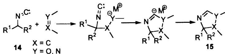
Scheme 6
