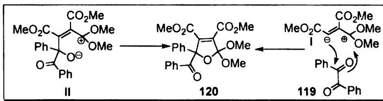
Scheme 35
