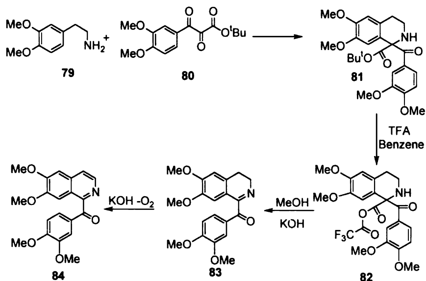
Scheme 27
