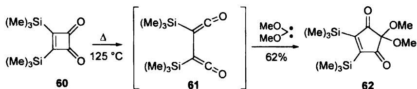
Scheme 15
