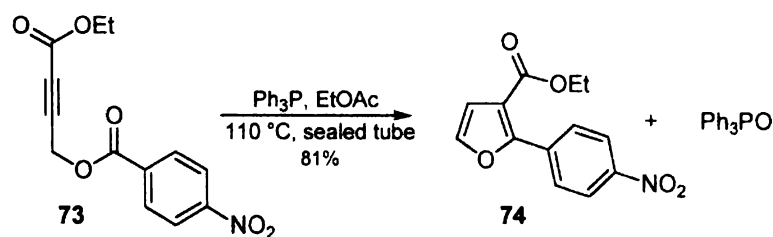
Scheme 26
