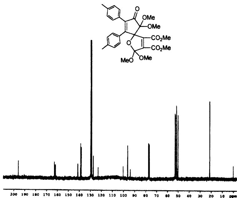
Figure 5 ^{13}\text{C} NMR spectrum of compound 134
