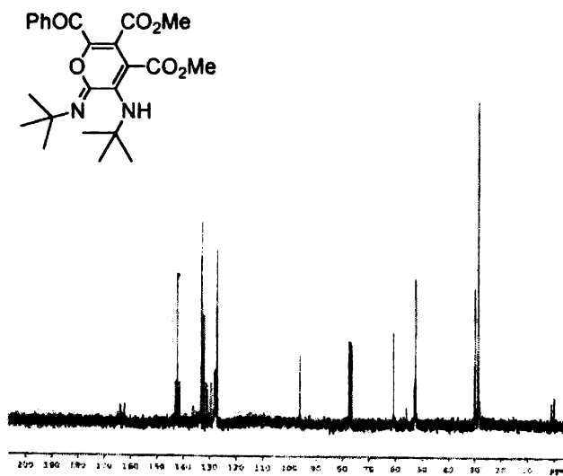
Figure 6 13 C NMR spectrum of compound 121
