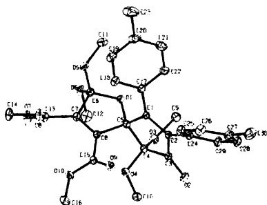
Figure 6 Single crystal X-ray structure of 134
