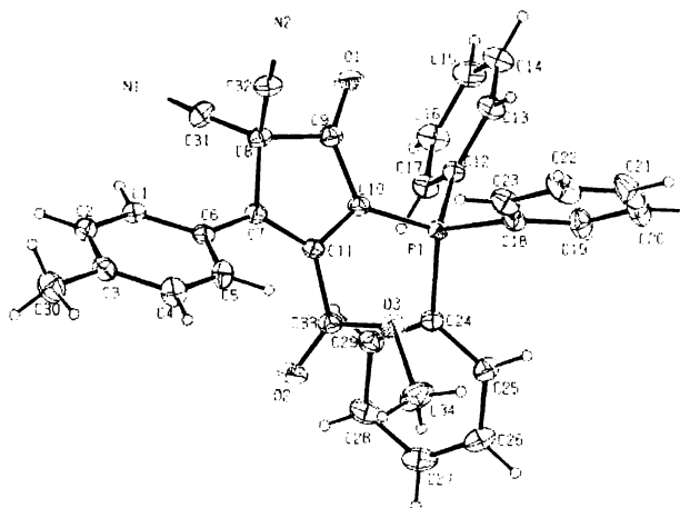
Figure 3 Single X-ray crystal structure of 76
