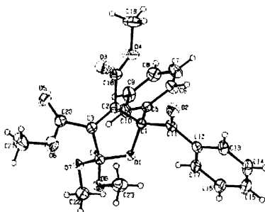
Figure 3 Single crystal X-ray structure of 120
