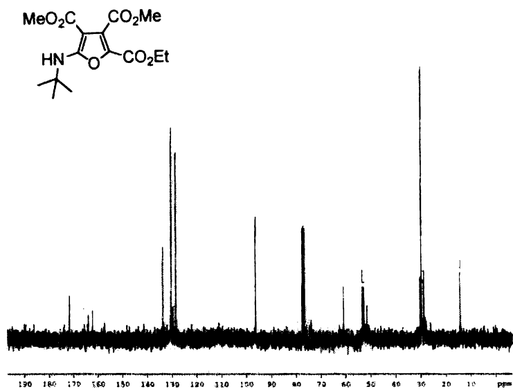
Figure 4 13 C NMR spectrum of compound 111
