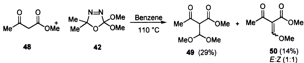
Scheme 11
