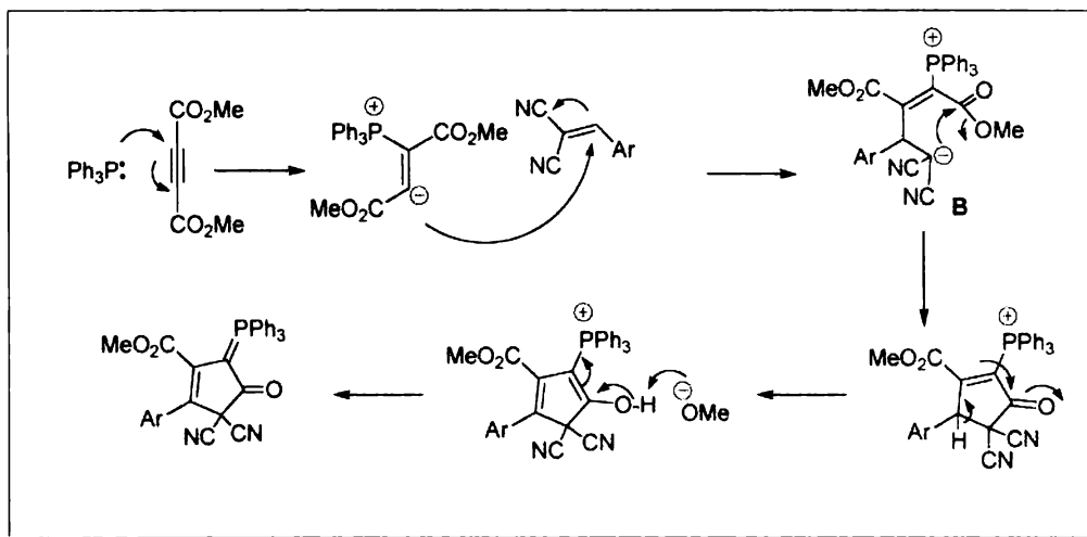
Scheme 32
