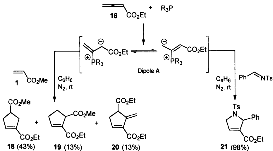
Scheme 8
