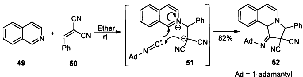
Scheme 20
