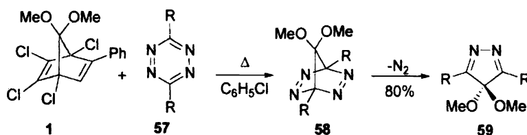
Scheme 14
