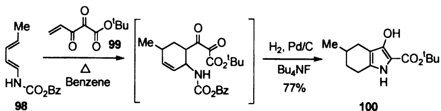
Scheme 32
