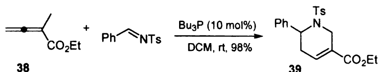
Scheme 14
