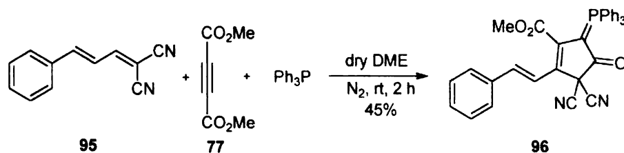
Scheme 30
