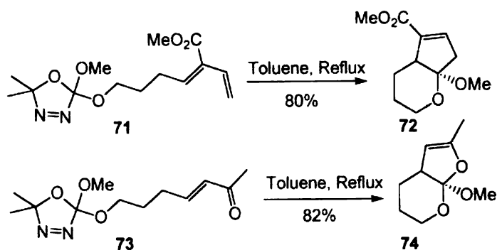
Scheme 18
