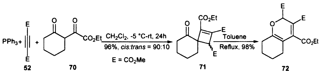
Scheme 25
