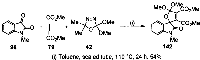
Scheme 40
