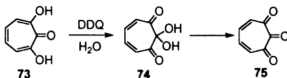
Scheme 25
