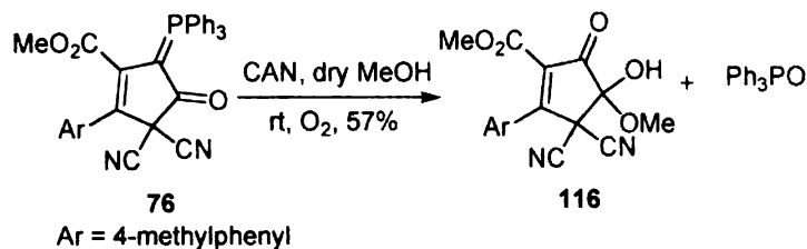
Scheme 33
