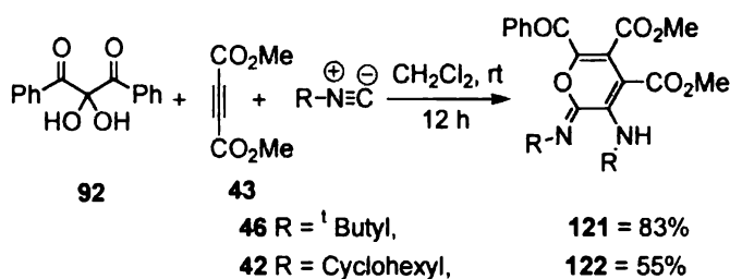
Scheme 36
