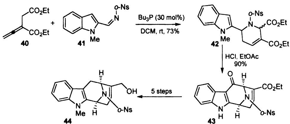
Scheme 15
