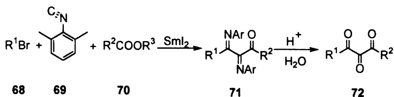
Scheme 24
