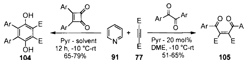
Scheme 32
