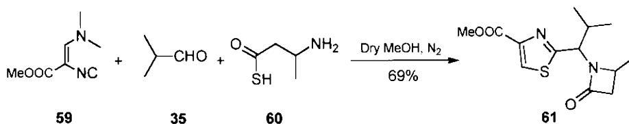
Scheme 18
