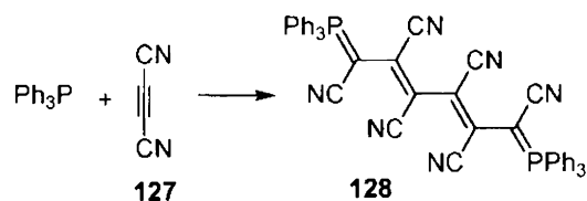
Scheme 41
