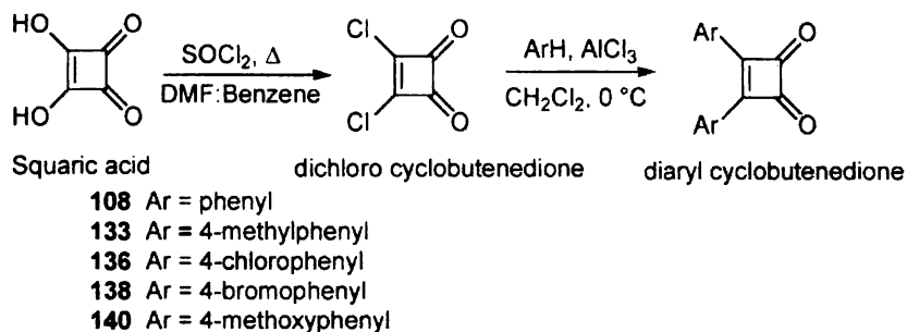
Scheme 36
