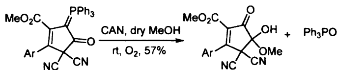
Scheme 3
