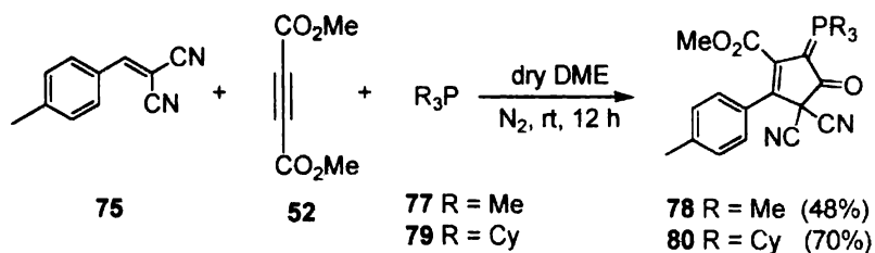
Scheme 29
