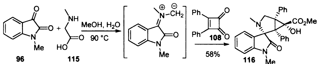
Scheme 30
