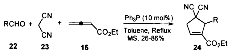
Scheme 9
