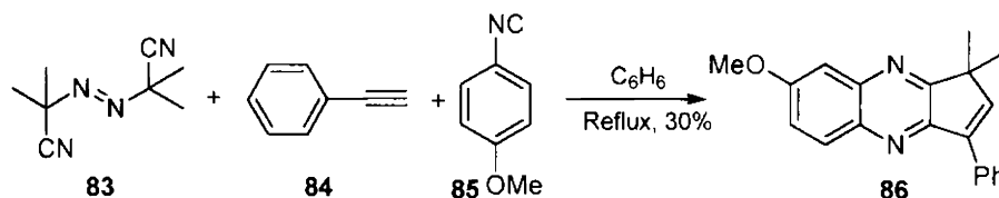
Scheme 25
