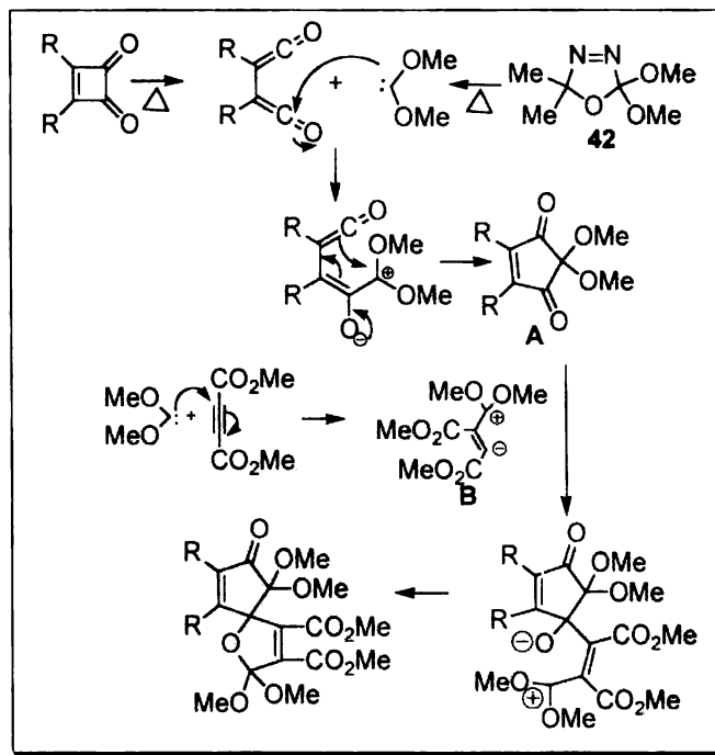
Scheme 38
