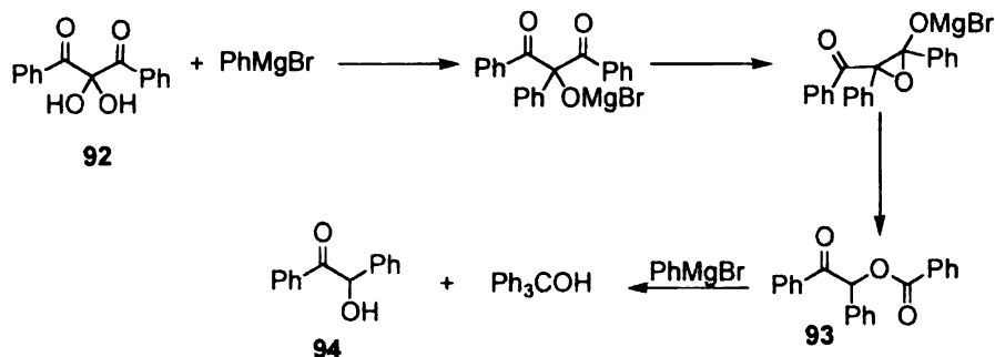
Scheme 30
