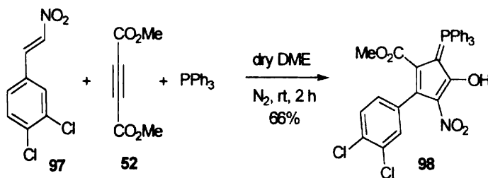
Scheme 31
