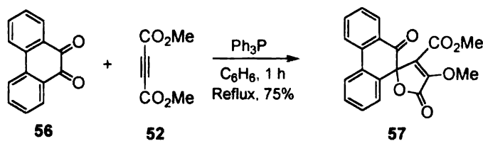
Scheme 20
