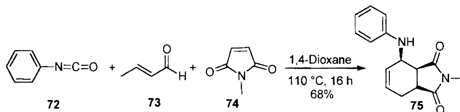
Scheme 22
