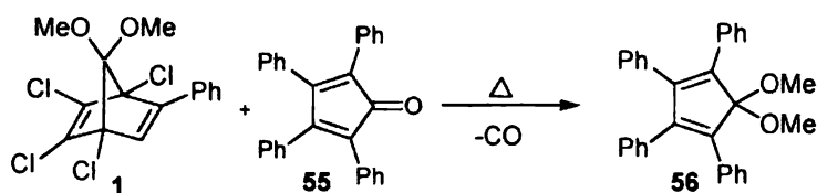
Scheme 13
