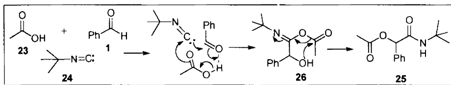
Scheme 9
