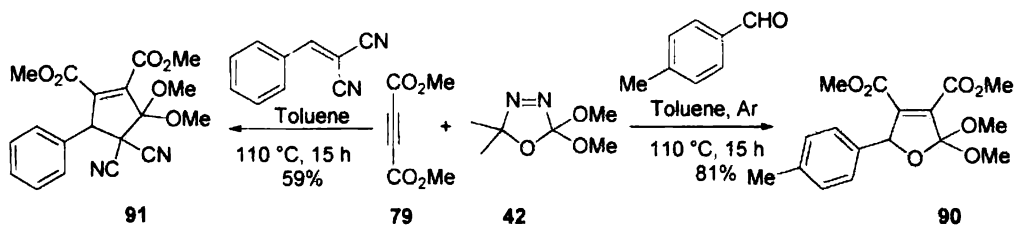
Scheme 23
