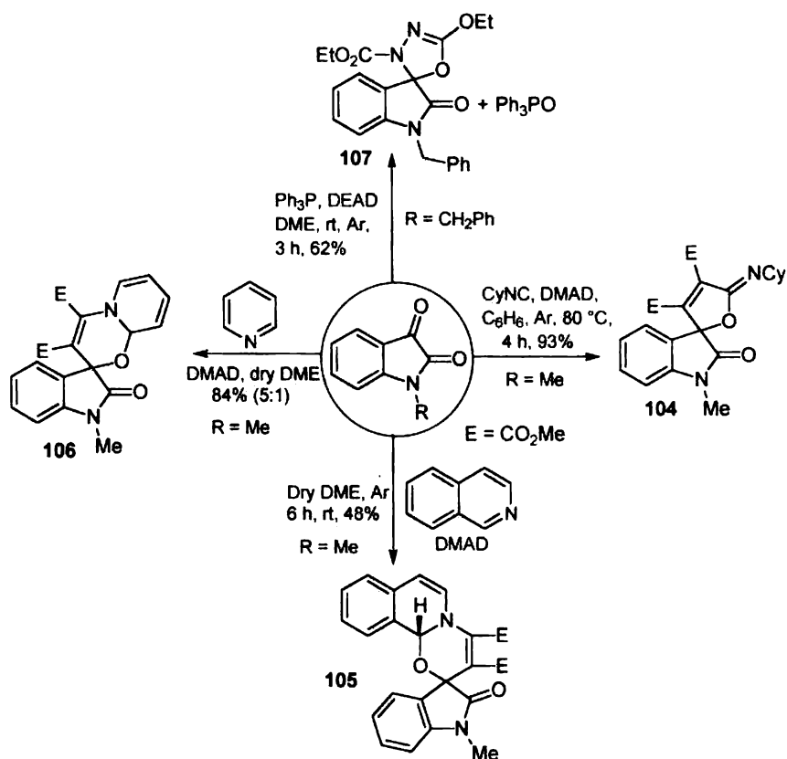
Scheme 27
