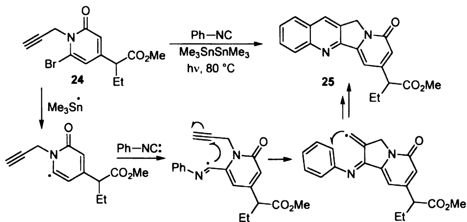
Scheme 11
