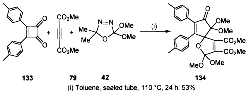
Scheme 37
