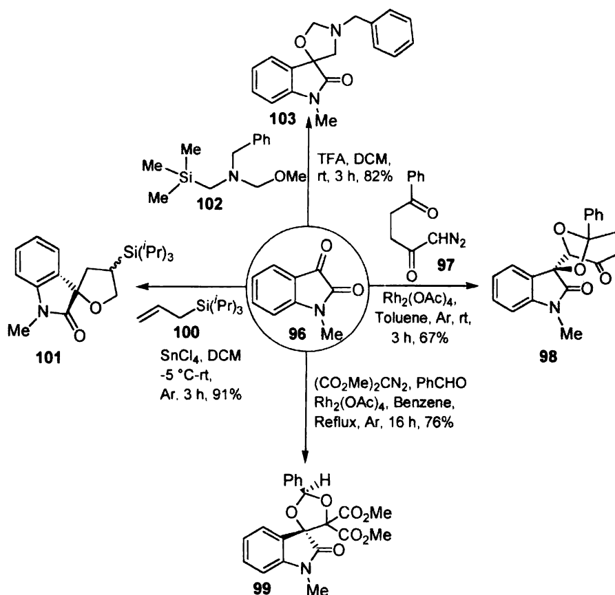
Scheme 26
