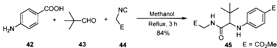
Scheme 15
