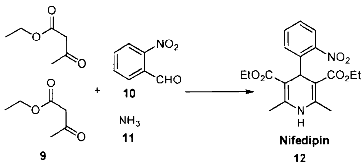
Scheme 4
