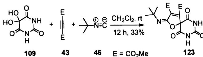
Scheme 38
