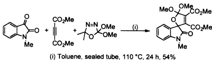
Scheme 5
