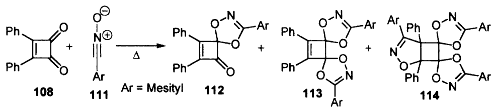
Scheme 29
