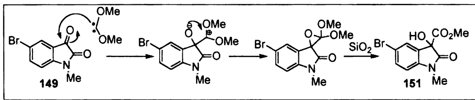
Scheme 41
