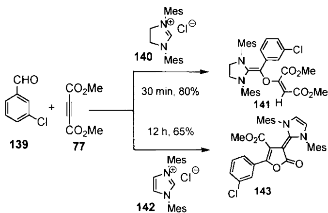
Scheme 47
