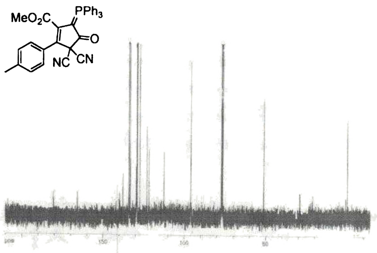
Figure 2 13 C NMR spectrum of 76
