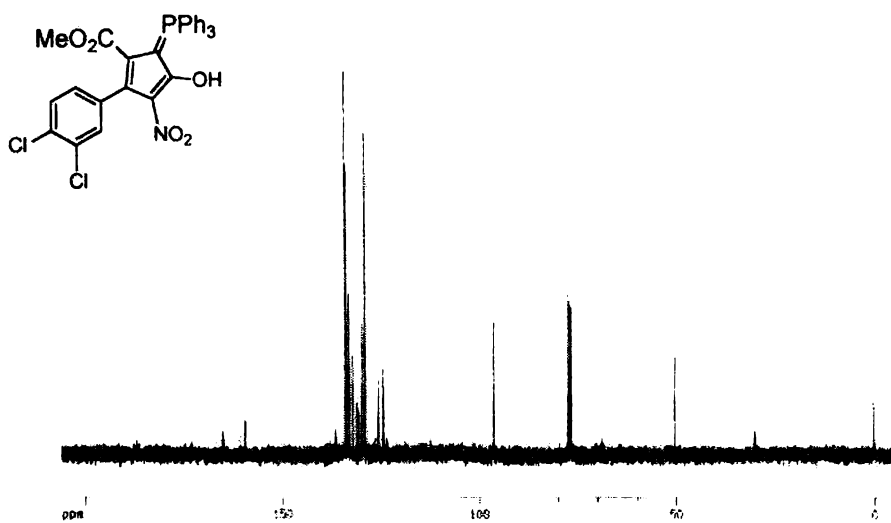
Figure 5 ^{13}\text{C} NMR spectrum of 98
