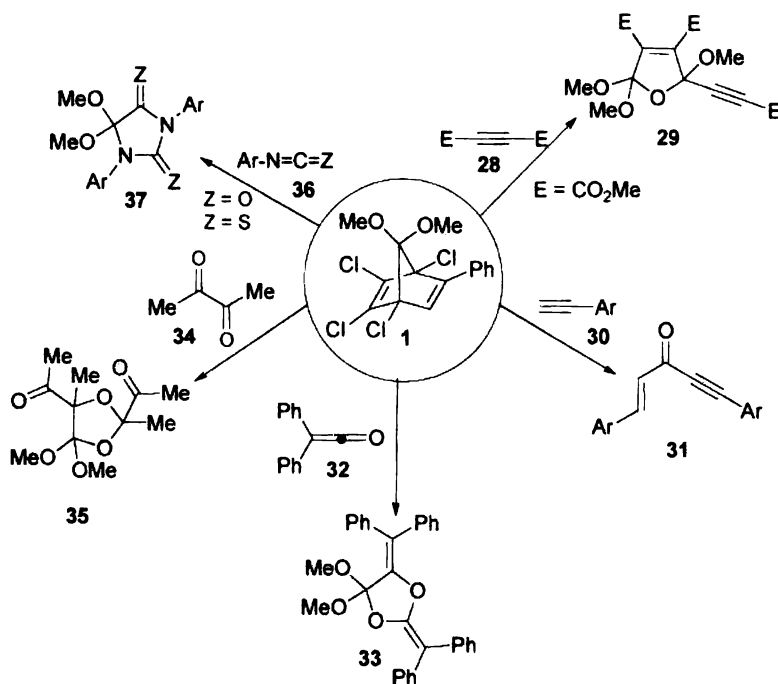
Scheme 8
