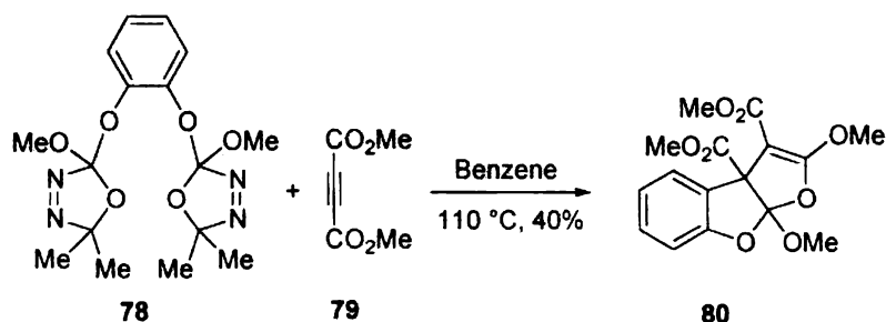
Scheme 20
