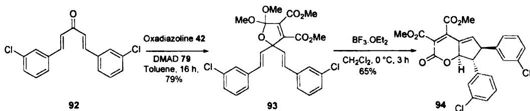
Scheme 24
