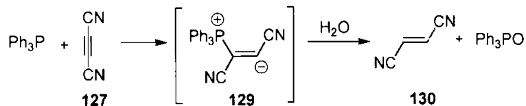
Scheme 42
