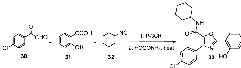
Scheme 11
