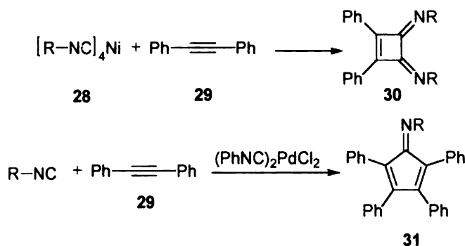
Scheme 13
