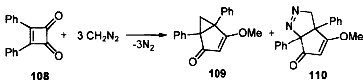
Scheme 28
