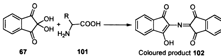
Scheme 33
