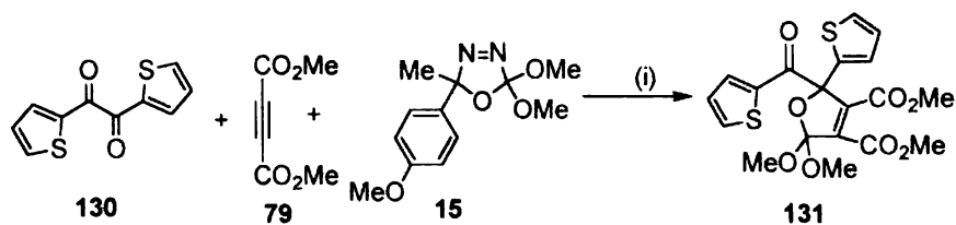
Scheme 34
