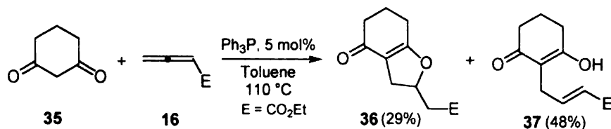
Scheme 13
