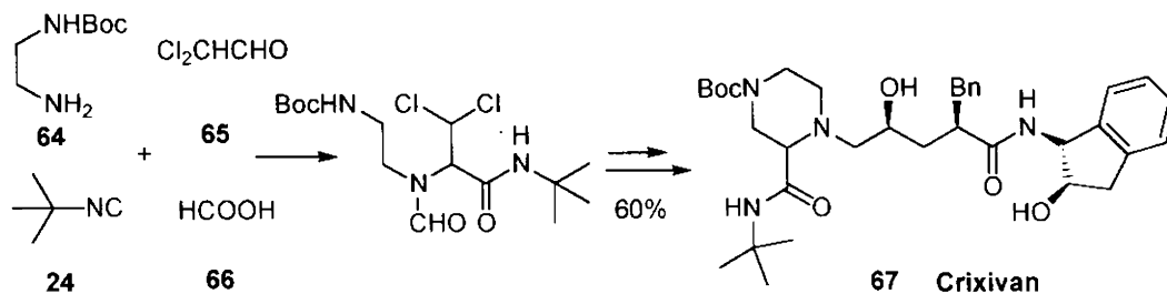
Scheme 20
