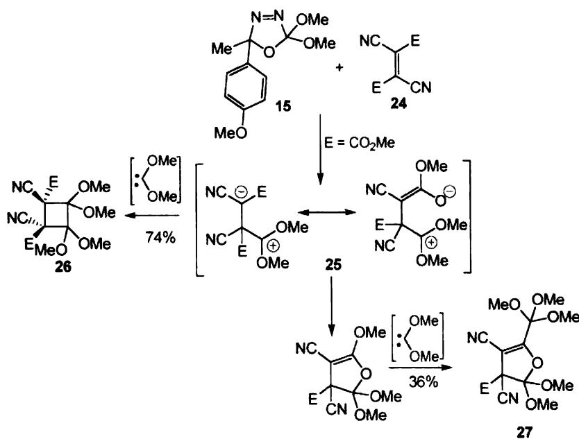
Scheme 7
