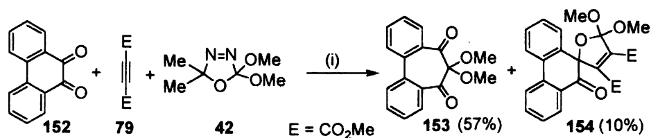
Scheme 42
