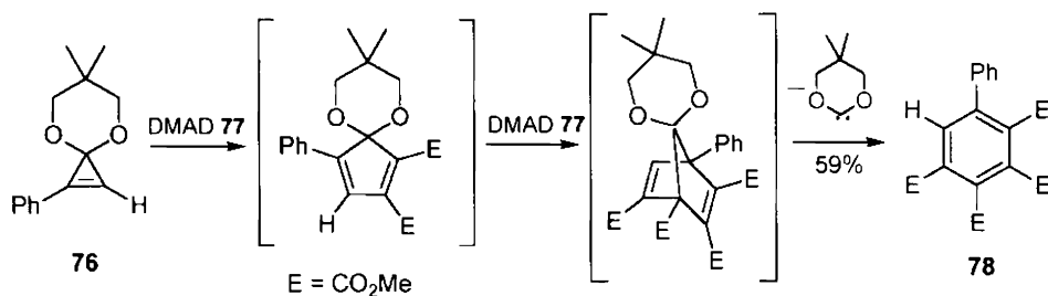
Scheme 23
