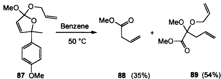
Scheme 22
