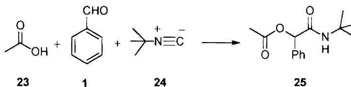
Scheme 8
