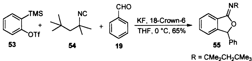
Scheme 21
