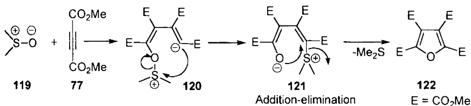
Scheme 39
