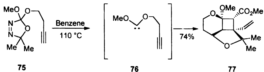
Scheme 19
