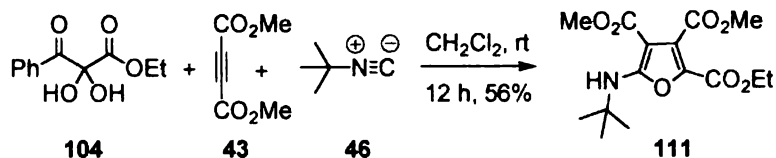
Scheme 35
