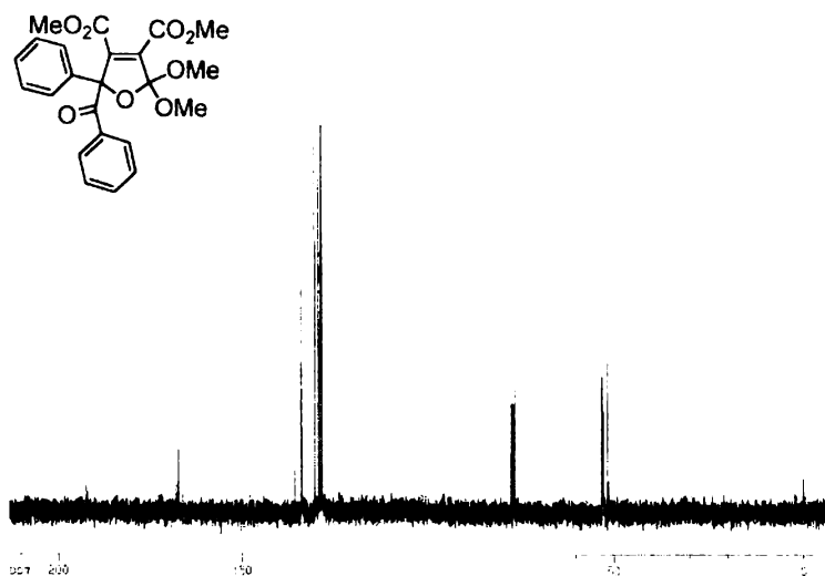
Figure 2 ^{13}\text{C} NMR spectrum of compound 120
