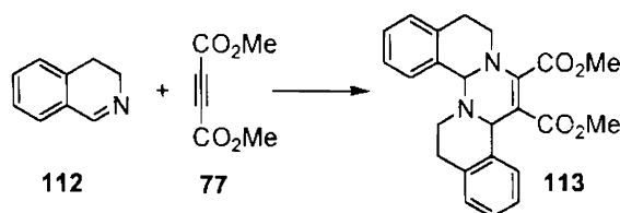
Scheme 36
