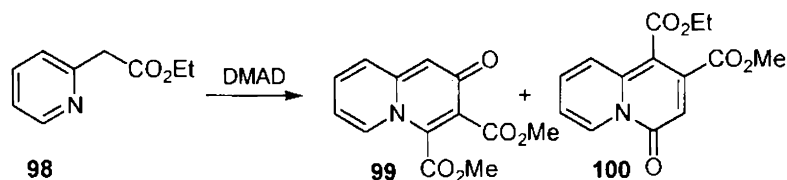
Scheme 29
