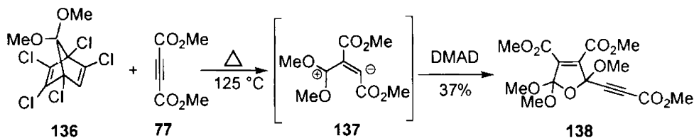
Scheme 46
