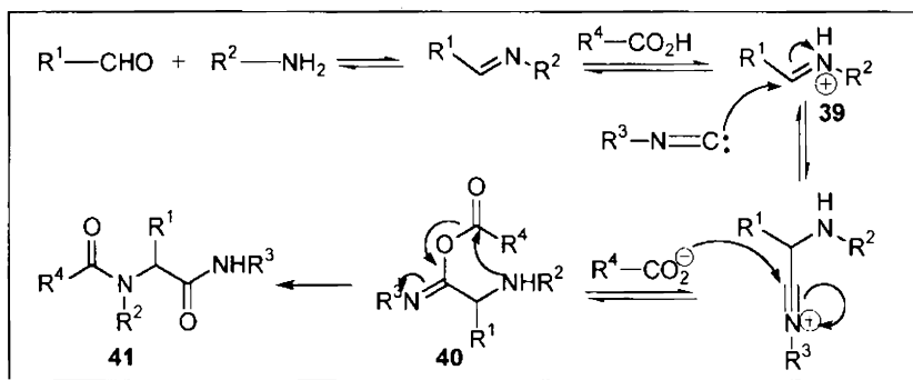
Scheme 14
