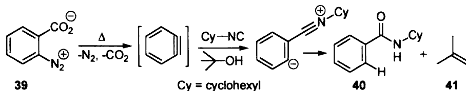
Scheme 17
