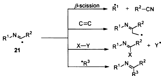
Scheme 9
