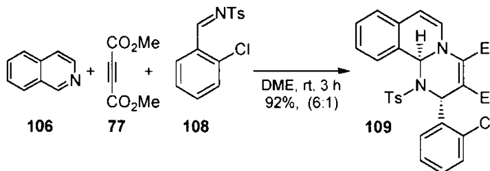
Scheme 34
