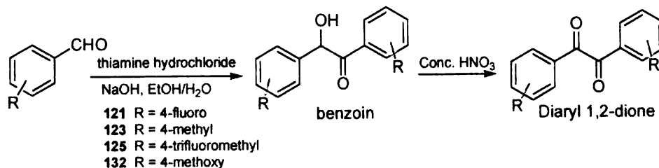
Scheme 32
