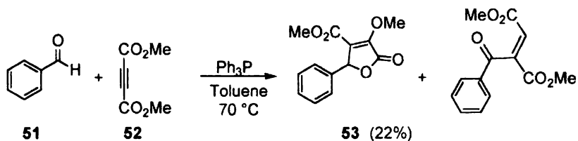
Scheme 18
