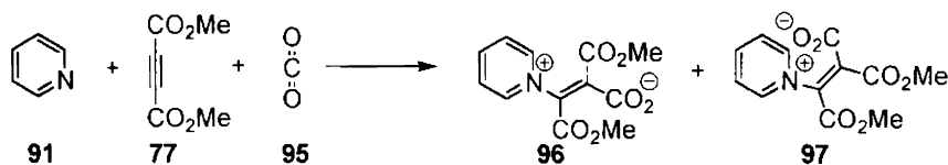
Scheme 28
