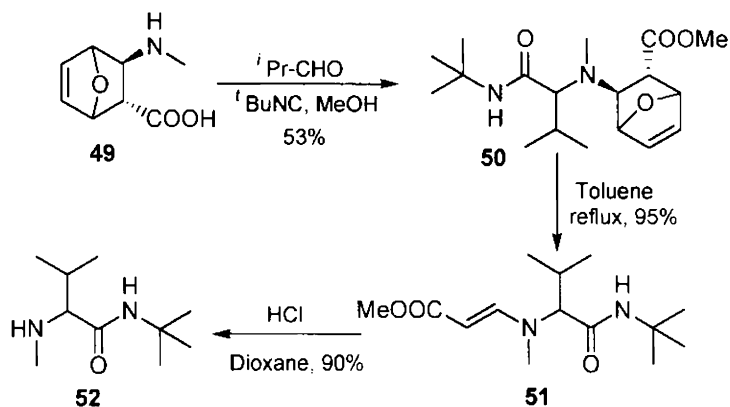
Scheme 16
