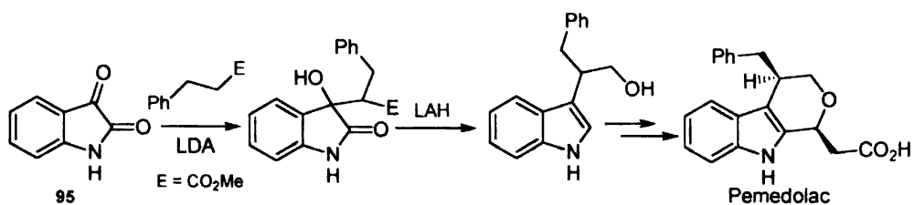
Scheme 25
