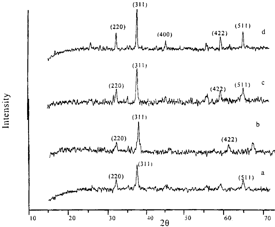
Fig.8.1: X-ray diffraction pattern of the (a) as prepared \text{Li}_{0.5}\text{Fe}_{2.5}\text{O}_4 powder, (b) the \text{Li}_{0.5}\text{Fe}_{2.5}\text{O}_4 powder heated at 300°C. (c) at 600°C and (d) 900°C
