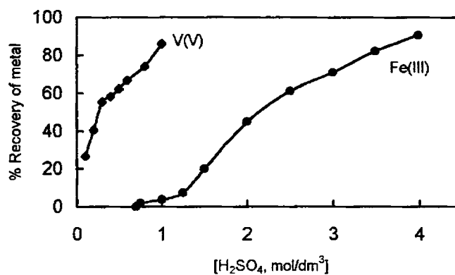
Figure 4.11 Stripping behaviour of vanadium(V), iron(III) and titanium(IV) from loaded EHEHPA ( 0.5 \text{ mol/dm}^3 ) phase using \text{H}_2\text{SO}_4 .
