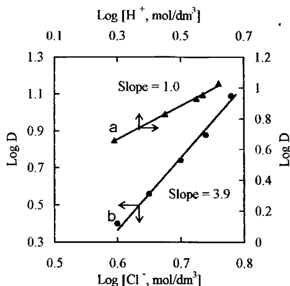
Figure 2.3 (a) Effect of hydrogen ion concentration on the extraction of iron(III); [\text{FeCl}_3] = 1 \text{ mol/dm}^3 , [\text{Cl}^-] = 5 \text{ mol/dm}^3 . (b) Effect of chloride ion concentration on the extraction of iron(III); [\text{FeCl}_3] = 1 \text{ mol/dm}^3 , [\text{H}^+] = 2 \text{ mol/dm}^3 .
