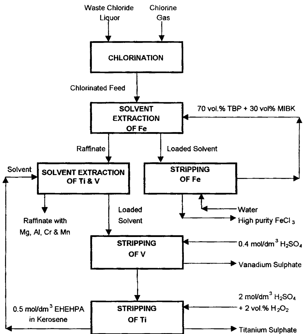
Figure 5.1 Schematic flow diagram for the two step solvent extraction process.
