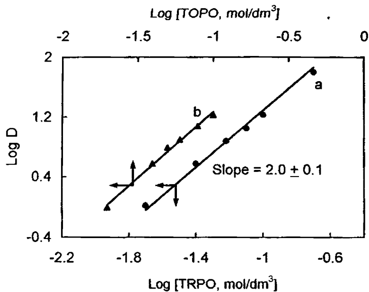
Figure 2.11 Effect of extractant concentration on the extraction of iron(III). Aq. ph.: [\text{Fe(III)}] = 3.6 \times 10^{-4} \text{ mol/dm}^3 , [\text{HCl}] = 2.0 \text{ mol/dm}^3 , Org. ph.: (a) TRPO (b) TOPO.
