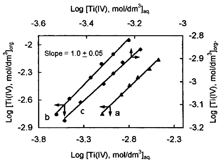
Figure 3.7 Effect of metal ion concentration on the extraction of titanium(IV). (a) [EHEHPA] = 0.1 mol/dm 3 , [HCl] = 1.0 mol/dm 3 (b) [BTMPPA] = 0.05 mol/dm 3 , [HCl] = 0.18 mol/dm 3 (c) [BTMPTPA] = 0.1 mol/dm 3 , [HCl] = 0.1 mol/dm 3 .
