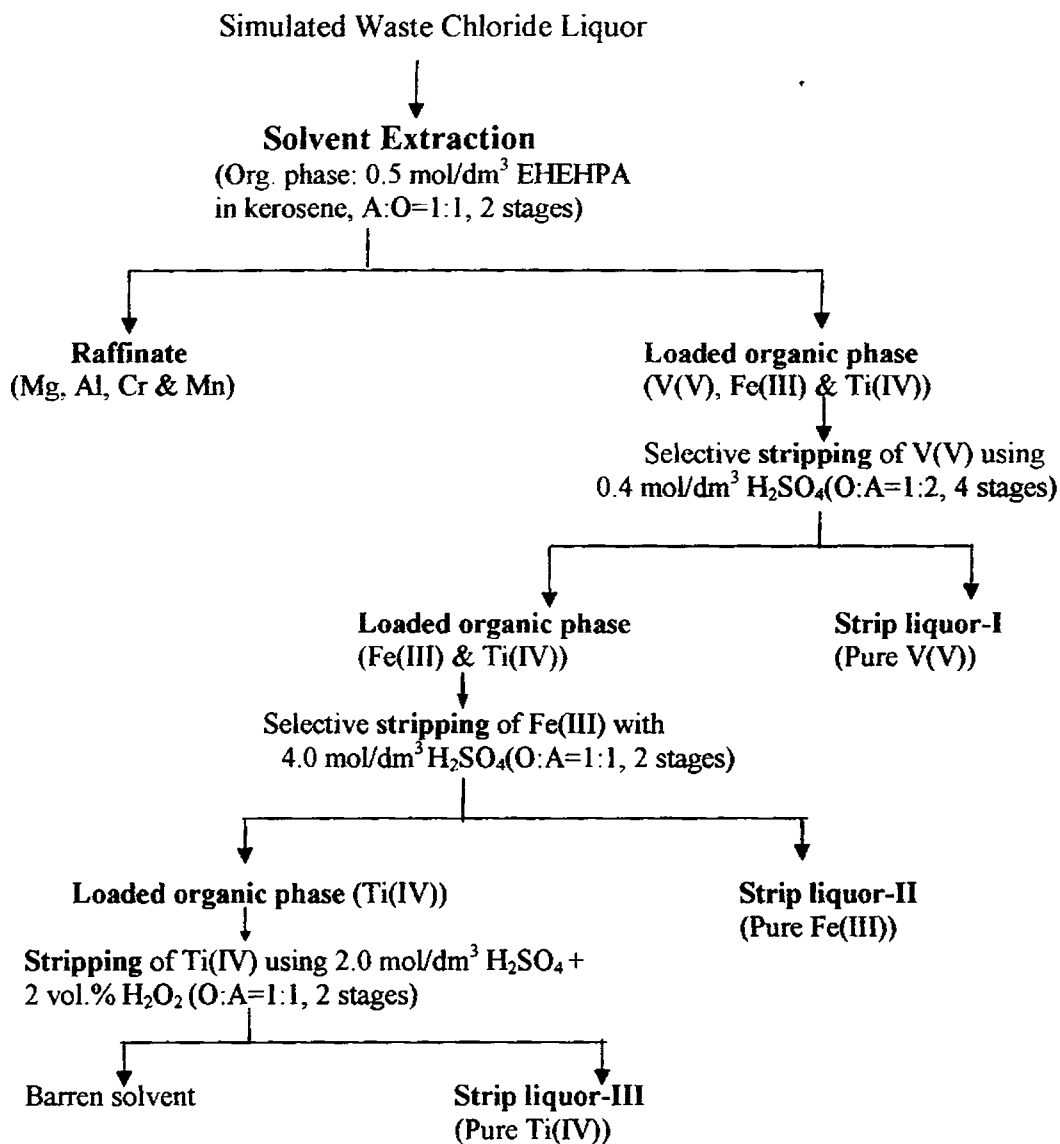
Figure 4.12 Separation scheme for the recovery of vanadium(V) from simulated titania waste chloride liquor.
