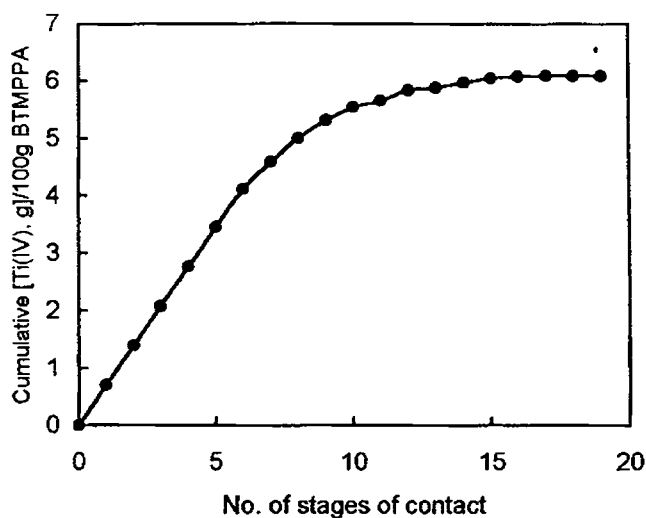
Figure 3.11 Loading of BTMPPA by titanium(IV). [\text{BTMPPA}] = 0.2 \text{ mol/dm}^3 , [\text{HCl}] = 0.25 \text{ mol/dm}^3 .
