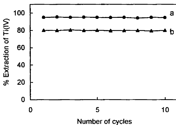
Figure 3.12 Recycling capacity of extractants. (a) [EHEHPA] = 0.2 mol/dm 3 , [Ti(IV)] = 0.01 mol/dm 3 , [HCl] = 1.0 mol/dm 3 . (b) [BTMPPA] = 0.05 mol/dm 3 , [Ti(IV)] = 2.5 × 10 -3 mol/dm 3 , [HCl] = 0.14 mol/dm 3 .
