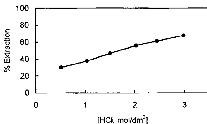
Figure. 2.2 Extraction behaviour of iron(III) ( 1 \text{ mol/dm}^3 ) using 70 vol.% TBP and 30 vol.% MIBK mixed solvent system from hydrochloric acid solutions.
