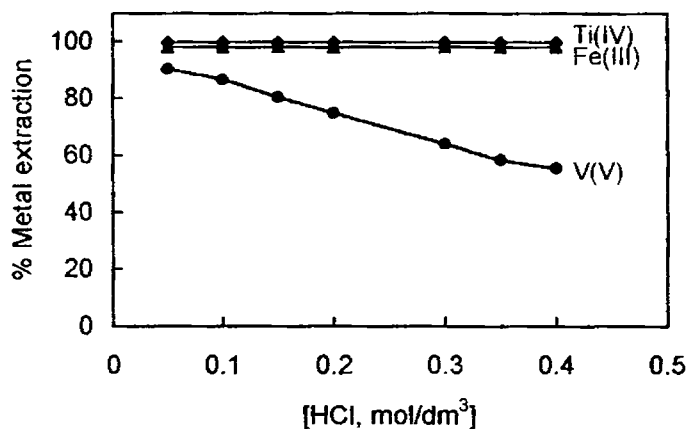
Figure 4.10 Extraction behaviour of titanium(IV), vanadium(V), and iron(III) using EHEHPA ( 0.5 \text{ mol/dm}^3 ) in kerosene from hydrochloric acid solutions. [Metal ion] = 0.01 \text{ mol/dm}^3 .
