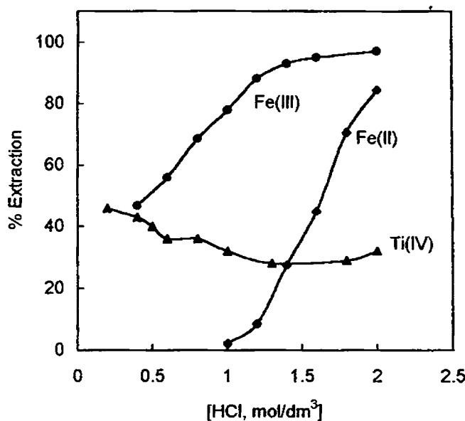
Figure 2.13 Effect of hydrochloric acid concentration on the extraction of iron(III) ( 3.6 \times 10^{-4} mol/dm 3 ), iron(II) ( 3.6 \times 10^{-4} mol/dm 3 ) and titanium(IV) ( 1 \times 10^{-3} mol/dm 3 ), using 0.2 mol/dm 3 TRPO in xylene.
