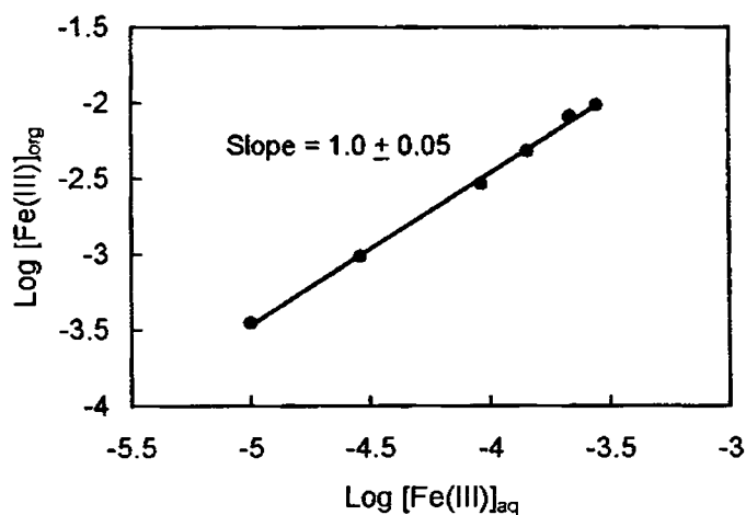
Figure 2.10 Effect of metal ion concentration on the extraction of iron(III) from 2.0 \text{ mol/dm}^3 HCl solutions using 0.2 \text{ mol/dm}^3 TRPO in xylene.
