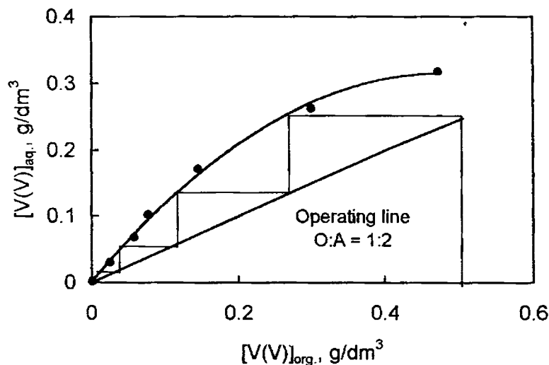
Figure 4.8 McCabe-Thiele plot for vanadium(V) stripping. [V(V)]_{org} = 0.51 \text{ g/dm}^3 , [H_2SO_4] = 0.4 \text{ mol/dm}^3 .
