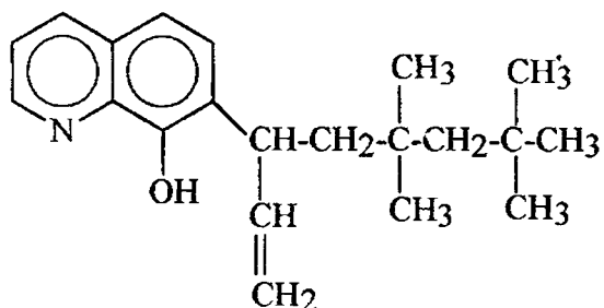
7-[3-(5,5,7,7-tetramethyl-1-octenyl)]-8-hydroxyquinoline (Kelex 100)
