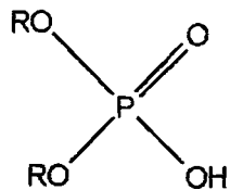
2. Dialkylphosphoric acid
