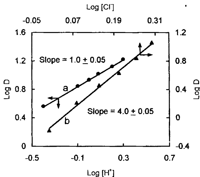
Figure 2.9 (a) Effect of hydrogen ion concentration on the extraction of iron(III). [\text{Fe(III)}] = 3.6 \times 10^{-4} \text{ mol/dm}^3 , [\text{Cl}^-] = 2.0 \text{ mol/dm}^3 . (b) Effect of chloride ion concentration on the extraction of iron(III), [\text{H}^+] = 1.0 \text{ mol/dm}^3 . Org. ph. : 0.1 \text{ mol/dm}^3 TRPO in xylene.
