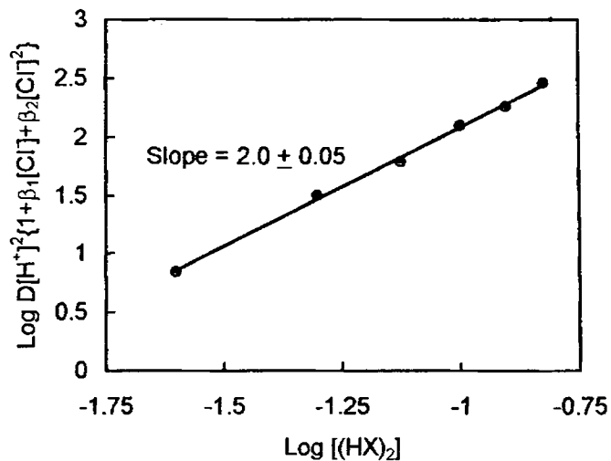
Figure 3.3 Effect of EHEHPA concentration on the extraction of titanium(IV). [Ti(IV)] = 0.01 mol/dm 3 , [HCl] = 1.0 mol/dm 3 .
