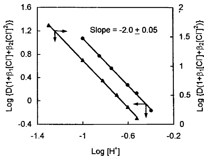
Figure 3.6 Effect of hydrogen ion concentration on the extraction of titanium(IV). (a) [BTMPPA] = 0.05 mol/dm 3 , [Ti(IV)] = 2.5 × 10 -3 mol/dm 3 (b) [BTMPTPA] = 0.2 mol/dm 3 , [Ti(IV)] = 1.0 × 10 -3 mol/dm 3 .
