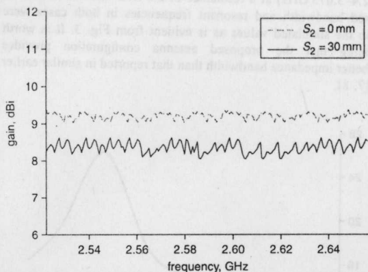
Fig. 5 Measured antenna gain against frequency
