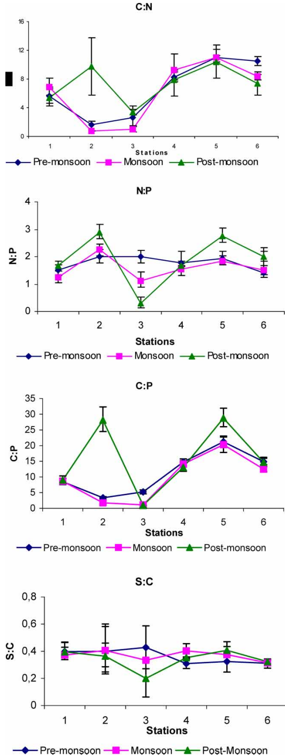
Figure 2. Seasonal and spatial variations of nutrient stoichiometry in the study region.
